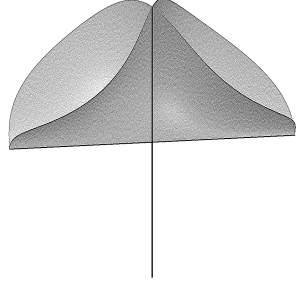
Figure 1.5: The front of the open Whitney umbrella
