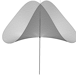
Figure 1.4: The ordinary Whitney umbrella in \mathbb{R}^3
