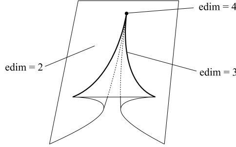
Figure 1.1: The open swallowtail \Sigma_2 \subset \mathbb{R}^4
