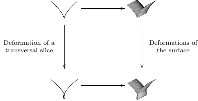
Figure 3.1: Propagation of deformations
