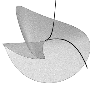
Figure 1.3: The front of the open swallowtail
