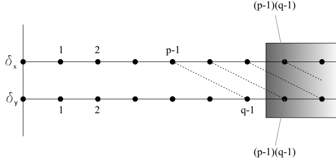
Figure 4.1: Monomial diagram
