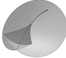
Figure 1.2: The ordinary swallowtail \Delta_2 \subset \mathbb{R}^3
