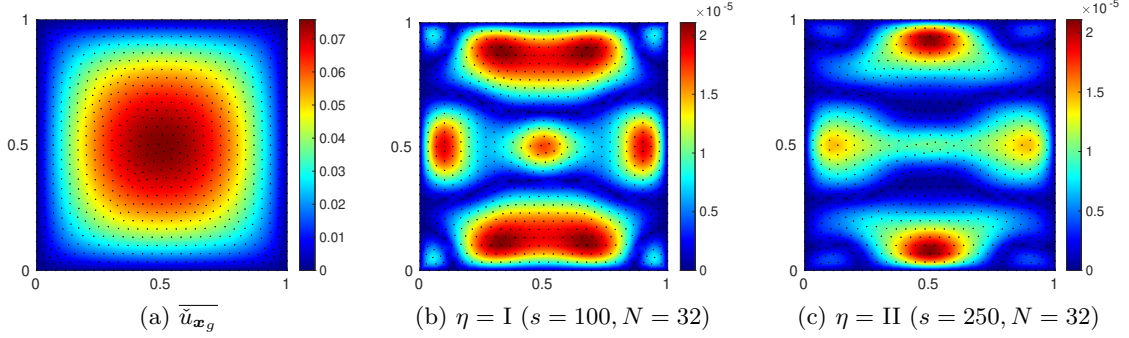
Figure 4.4: The MC approximation \overline{\tilde{u}_{\mathbf{x}_g}} and the pointwise errors |\overline{\tilde{u}_{\mathbf{x}_g}} - \mathbb{E}(u_{\mathbf{x}_g}^{\text{usFFT}})| for \eta = \text{I} and \text{II} for the affine example.
