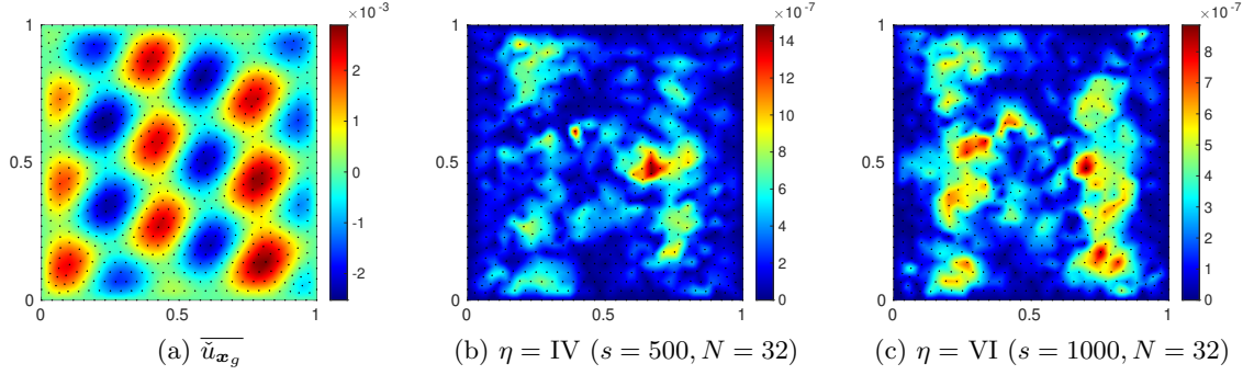
Figure 4.7: The MC approximation \bar{u}_{x_g} and the pointwise errors |\bar{u}_{x_g} - \mathbb{E}(u_{x_g}^{\text{usFFT}})| for \eta = \text{IV} and VI for the lognormal example.
