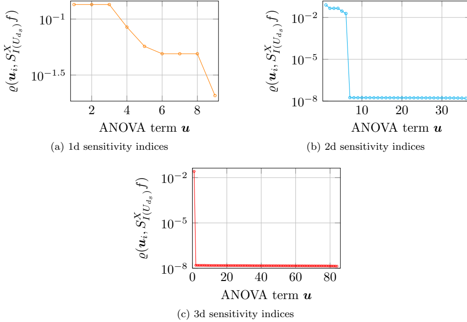
Fig. 4: Behavior of the global sensitivity indices \varrho(\mathbf{u}_i, S_{I(U_{d,s})}^X, f) for the example 8 from Table 1.
