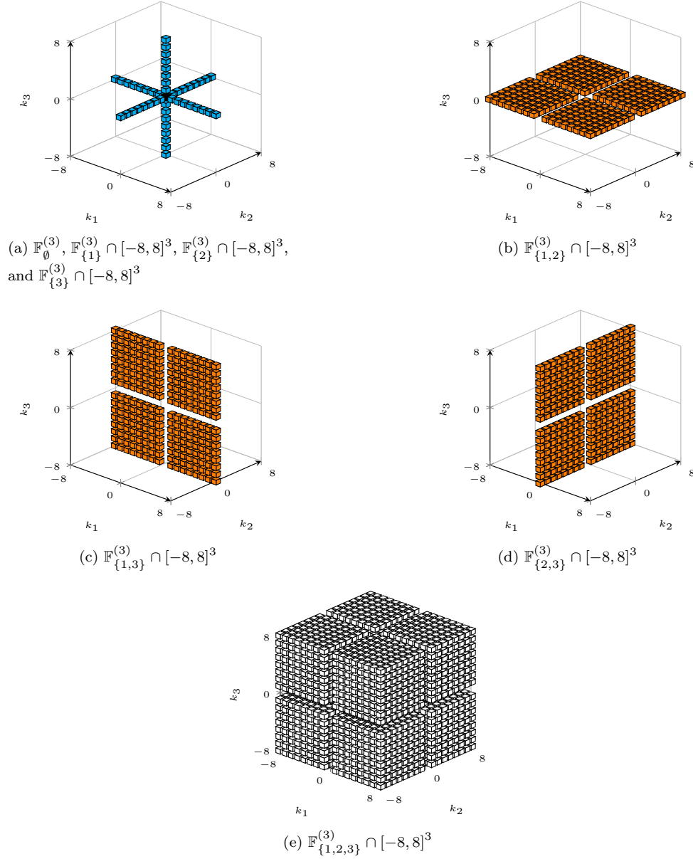
Fig. 1: The ANOVA decomposition working on the hypercube [-8, 8]^3 as a part of the 3-dimensional index set \mathbb{Z}^3 .
