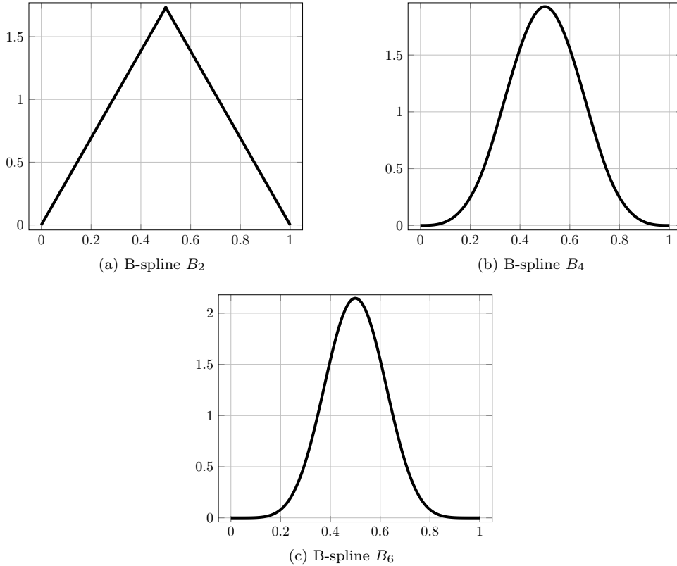
Fig. 3: B-splines B_2 , B_4 , and B_6 over \mathbb{T} \cong [0, 1) .
