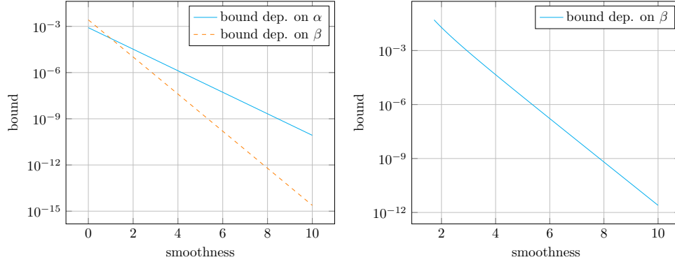
(a) bounds (4.8), (4.7) for 0 \leq \alpha \leq 10 , \beta = 1 (solid), and for \alpha = 1 , 0 \leq \beta \leq 10 (dashed) (b) bound (4.10) with \alpha = 0 , 1.7287 \leq \beta \leq 10 (solid)
