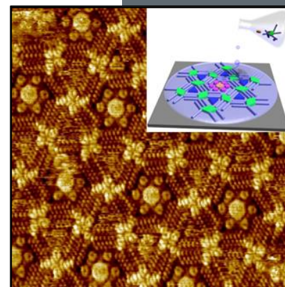
Complex self-assembled pattern containing triangular and hexagonal pores arranged around different combinations of template molecules
