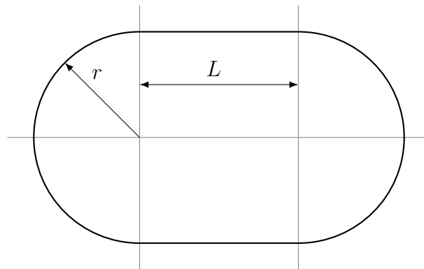
Figure 1: Stadium billiard
