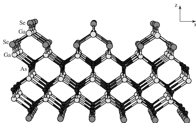
Figure 2. Lateral view of structure 3B in figure 1. z and x correspond to the [001] and [1\bar{1}0] crystallographic directions. Notice the presence of Se chains (each Se atom is bonded to two of the Ga atoms below) in the [110] direction.
