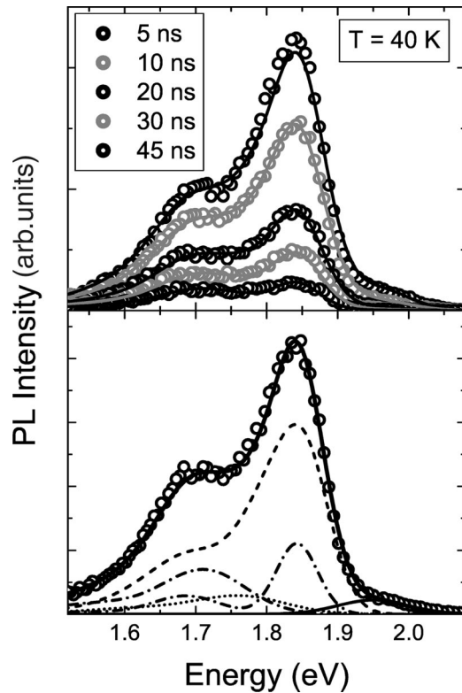
FIG. 2. Upper: evolution of the \alpha -PTCDA PL spectra measured at T = 40 K as a function of delay after the excitation pulse (circles). Each trace for a given delay t corresponds to a time integration over an interval of 2.5 ns for a representative sample of delay times t = 5, 10, 20, 30 , and 45 ns. The solid lines represent the calculated curves based on our model for the time-dependent PL. Lower: decomposition of the PL spectra integrated between delays of \sim 5 ns and 45 ns (circles) into the different recombination channels, with the Frenkel component (dashed line), the excimer band (dotted line), the two CT channels (dash-dotted line), and the sum of all components (solid line), including a high-energy band at 1.95 eV (solid line).
