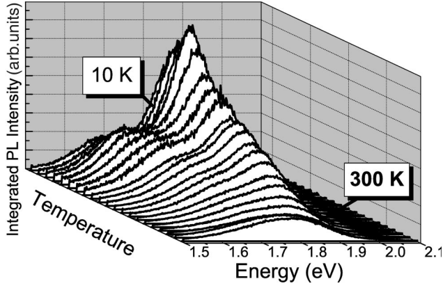
FIG. 1. Time-integrated PL spectra (delay – 5 ns to 45 ns) measured on a single crystal of \alpha -PTCDA, at different temperatures T = 10, 15, 20, 30, 40, 60, 80, 100, 125, 150, 160, 170, 180, 190, 200, 210, 225, 240, 260, 280 , and 300 K.
