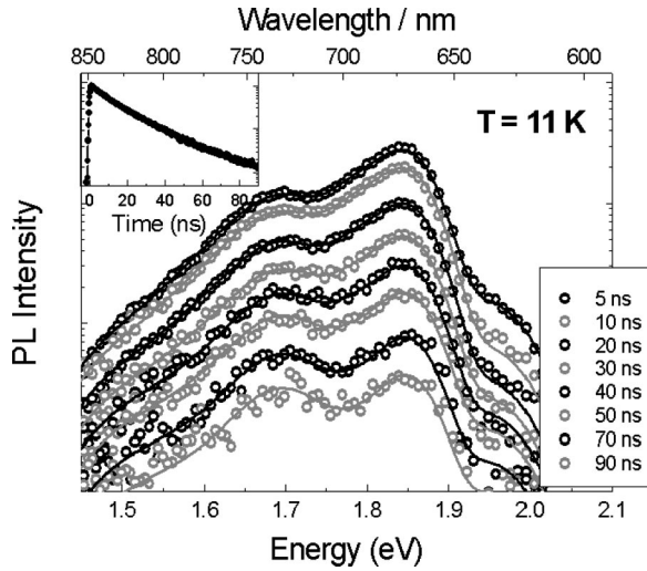
FIG. 1. Evolution of the PTCDA PL spectra as a function of delay after the excitation pulse (circles). The data are shown on a logarithmic scale, and each trace for a given delay t corresponds to a time-integration over an interval of 2.5 ns, i.e., (t-1.25 \text{ ns}, t+1.25 \text{ ns}) , for a representative sample of delay times t=5, 10, 20, 30, 40, 50, 70 , and 90 \text{ ns} . The solid lines represent the calculated curves based on our model for the time-dependent PL. For clarity, five consecutive spectral data points of the streak camera are summed up, resulting in 96 points with a sampling interval of 2.925 nm. The inset shows the decay of the PL intensity integrated over the whole spectral range on a logarithmic scale.
