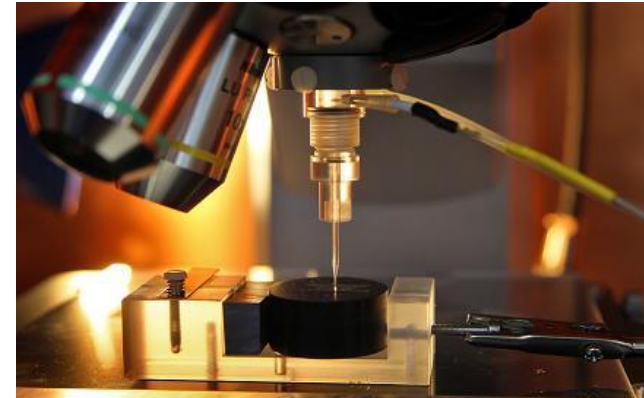
microcorrosion cell
