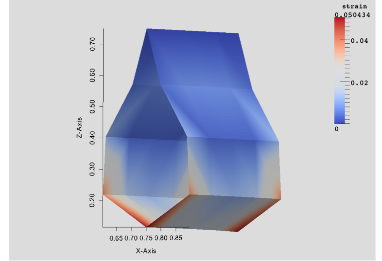
(a) 32 elements.
