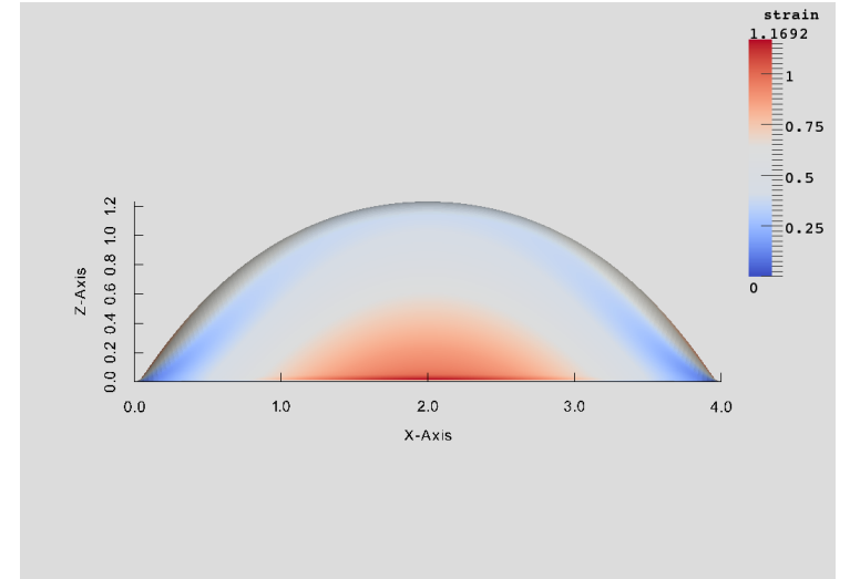
(b) 16384 elements.
