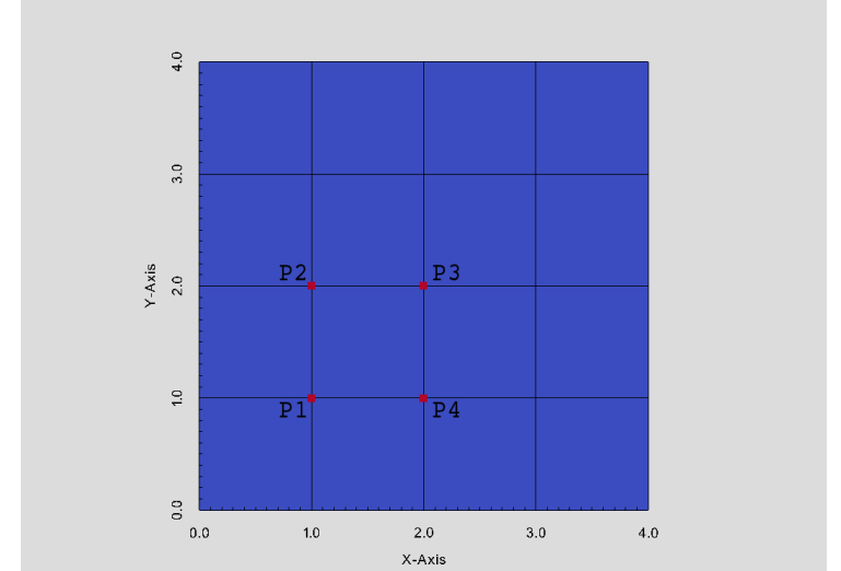
Figure 2: Position of the points for consideration of \mathbf{U} and \|\mathbf{E}\|_F .
