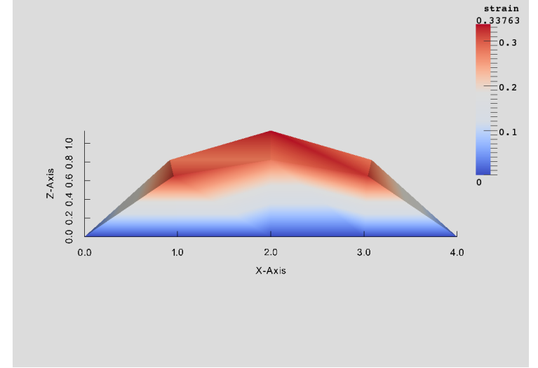
(a) 16 elements.
