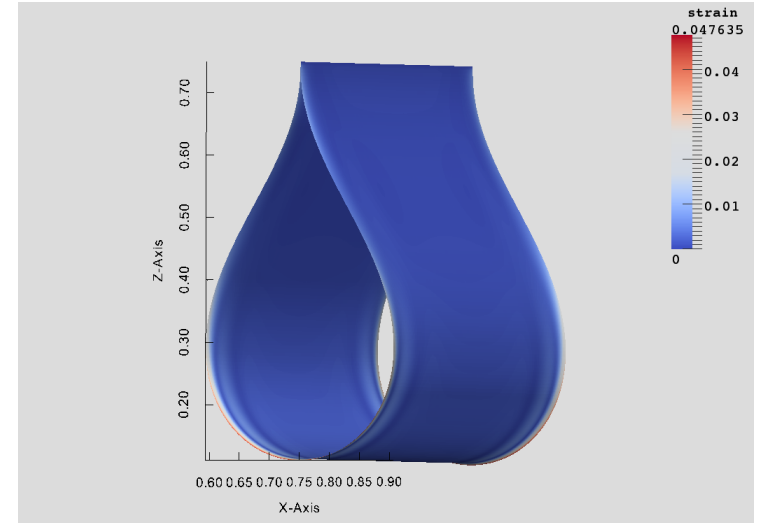
(b) 32768 elements.
