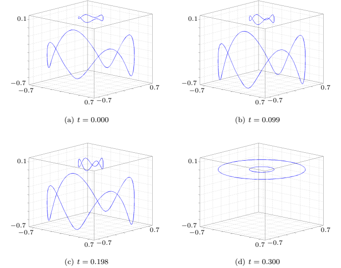
Figure 5.3: The computed control for the constrained control problem of Section 5.1 at different time steps.
