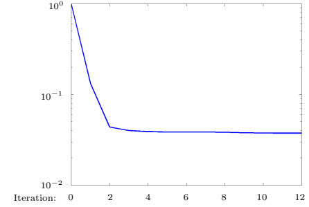
Figure 5.2: The relative cost functional \hat{J}(u^j)/\hat{J}(u^0) for the constrained control problem of Section 5.1.
