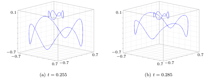
Figure 5.4: Activity of the control constraint the control problem of Section 5.1 at time steps t \in \{0.255, 0.285\} .
