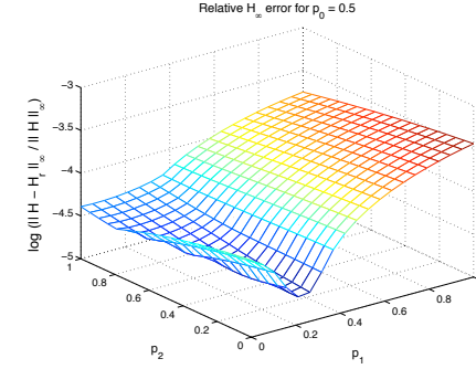
Figure 6: Example 6.1 with \nu = 3 : relative \mathcal{H}_\infty error as p_1 and p_2 vary.
