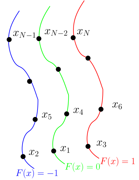
Figure 2: 2-d curve approximation
