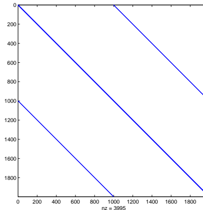
Figure 3.1: Sparsity pattern of test matrix
