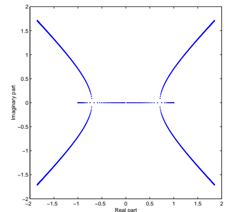
Figure 3.2: Spectrum of the test matrix
