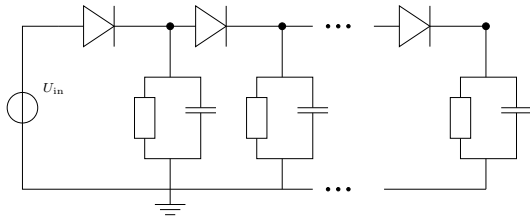
Figure 3: Diodechain [40].
