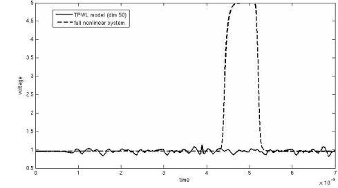
Figure 20: Inverter chain: TPWL-resimulation, reduction to order 50, repeated pulse, distance in full space, inverter 92.
