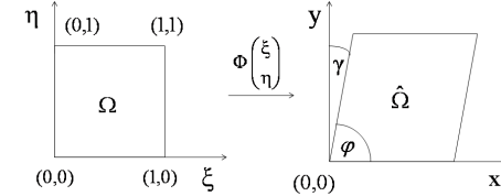
Figure 2: Transformation of unity square \Omega to deformed domain \hat{\Omega} by the use of mapping \Phi
