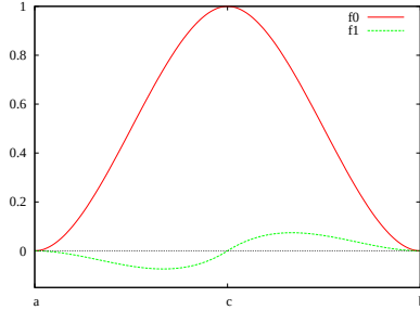
Figure 3: F(x)
