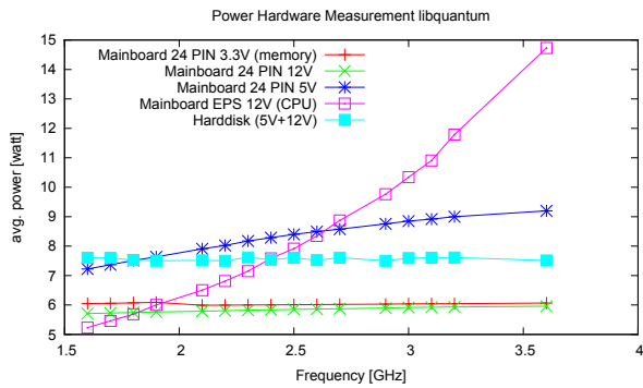
Figure 4: Detailed power measurement for the SPEC benchmark libquantum executed at different frequencies; measurement using the NI9205 device on an Intel Ivy Bridge processor.
