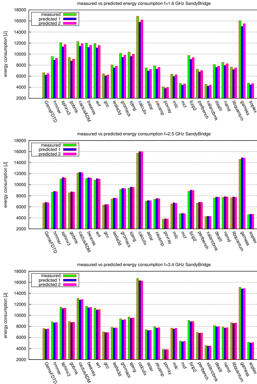
Figure 12: Intel Core i7 Sandy Bridge processor: Comparison of measured and predicted energy consumption of the SPEC CPU2006 integer and floating-point benchmarks for the frequencies f = 1.6 GHz (top), f = 2.5 GHz (middle), and f = 3.4 GHz (bottom).
