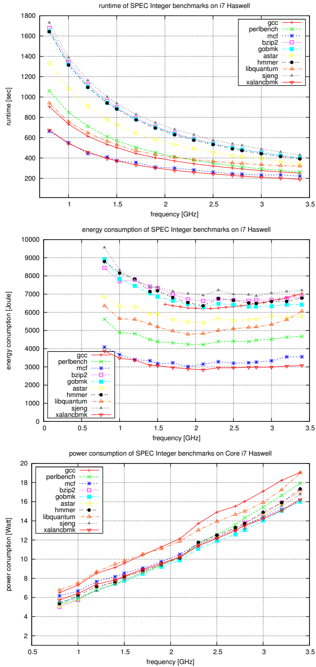
Figure 10: SPEC CPU2006 integer benchmarks on an Intel Core i7 Haswell processor: Runtime (top), energy consumption (middle), and power consumption (bottom) for varying frequencies.
