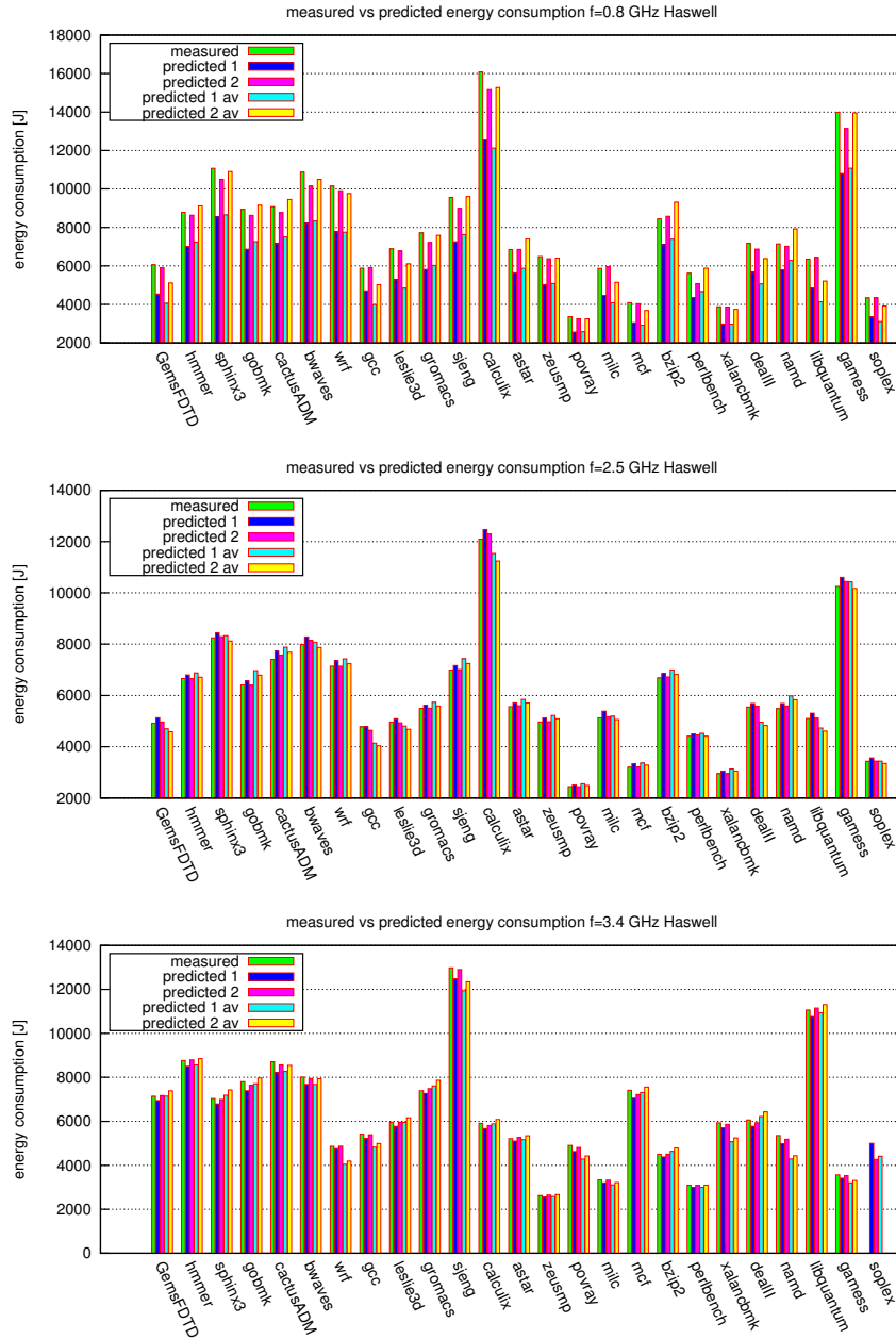
Figure 13: Intel Core i7 Haswell processor: Comparison of measured and predicted energy consumption of the SPEC CPU2006 integer and floating-point benchmarks for the frequencies f = 0.8 GHz (top), f = 2.5 GHz (middle), and f = 3.4 GHz (bottom).
