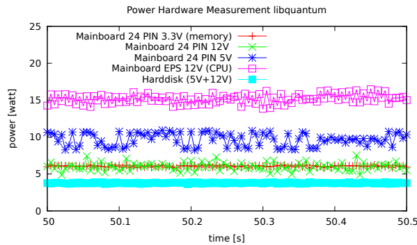
Figure 3: Detailed results of the power measurement for a specific time interval of the SPEC benchmark libquantum using the NI9205 device on an Intel Ivy Bridge processor.
