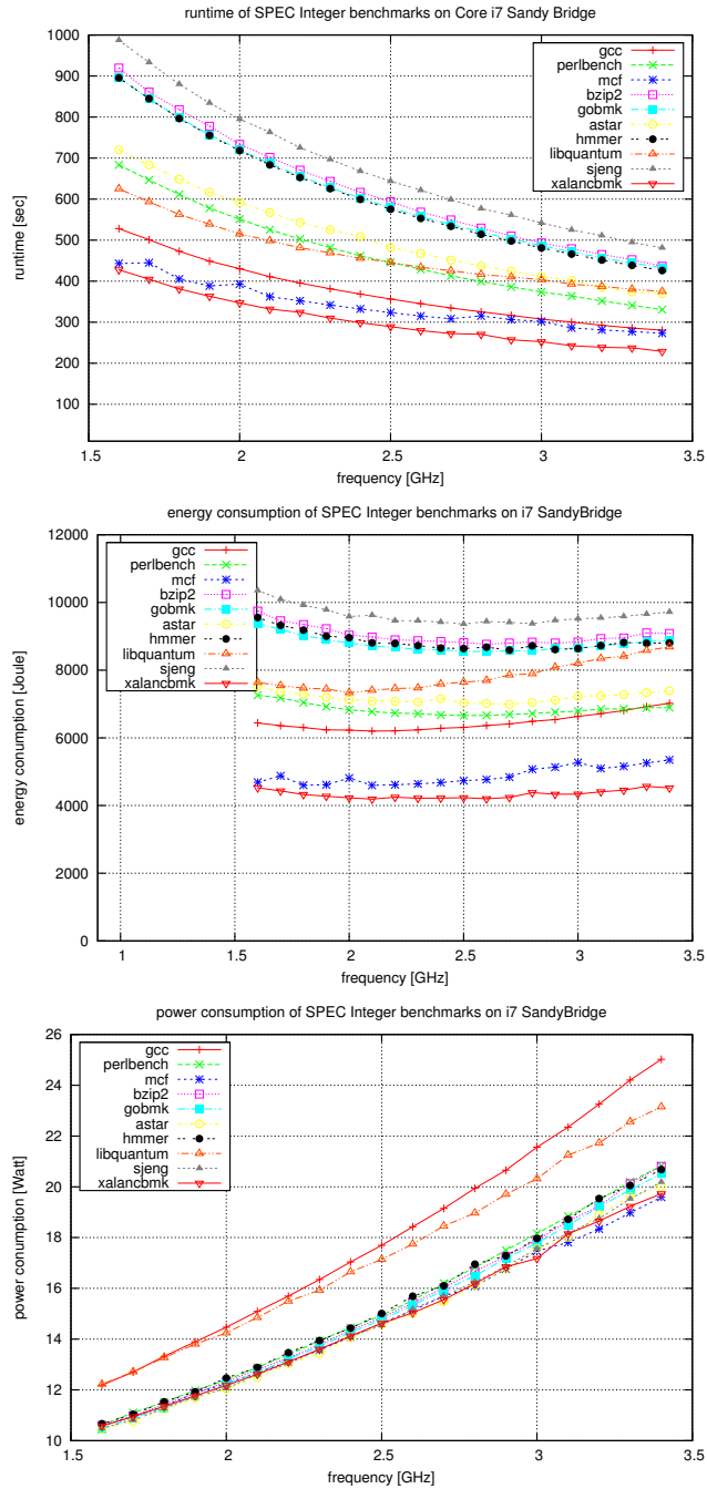
Figure 8: SPEC CPU2006 integer benchmarks on an Intel Core i7 Sandy Bridge processor: runtime (top), energy consumption (middle), and power consumption (bottom) for varying frequencies.
