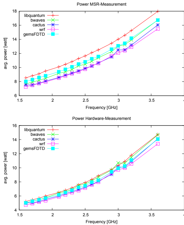
Figure 7: Comparison of power measurement with MSR registers (top) and NI9205 device (bottom) on an Intel Ivy Bridge processor.
