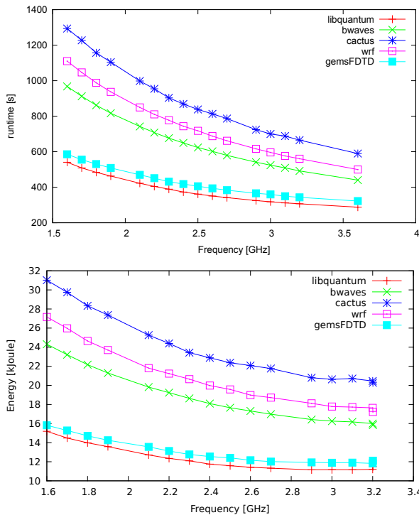
Figure 5: Runtime and energy consumption of selected SPEC CPU206 benchmarks with varying frequencies. For the energy, the total energy consumption is shown, collected with the NI9205 device on an Intel Ivy Bridge processor.
