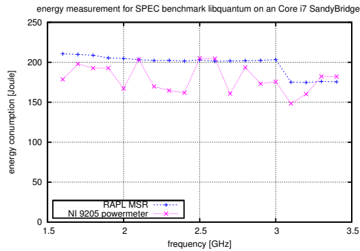
Figure 6: Comparison of the results of the energy measurement with power-meters and the energy measurement using RAPL for the SPEC benchmark libquantum on an Intel Core i7 Sandy Bridge processor.
