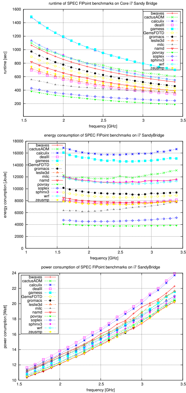
Figure 9: SPEC CPU2006 floating-point benchmarks on an Intel Core i7 Sandy Bridge processor: runtime (top), energy consumption (middle), and power consumption (bottom) for varying frequencies.
