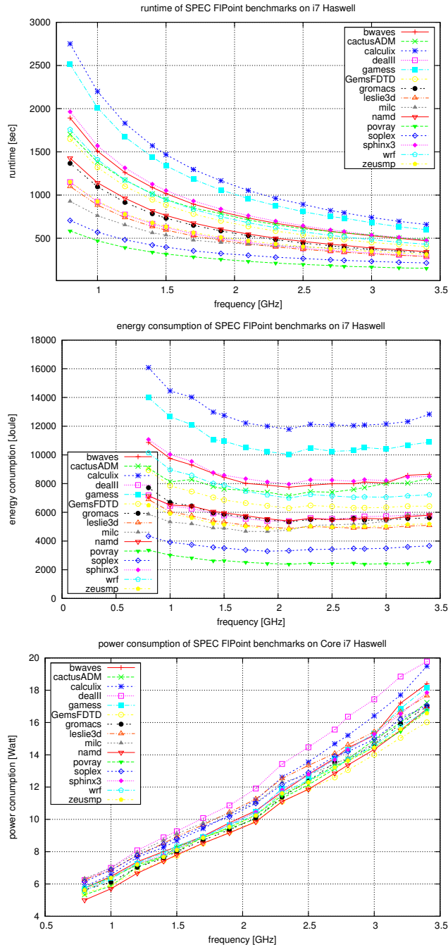
Figure 11: SPEC CPU2006 floating-point benchmarks on an Intel Core i7 Haswell processor: runtime (top), energy consumption (middle), and power consumption (bottom) for varying frequencies.
