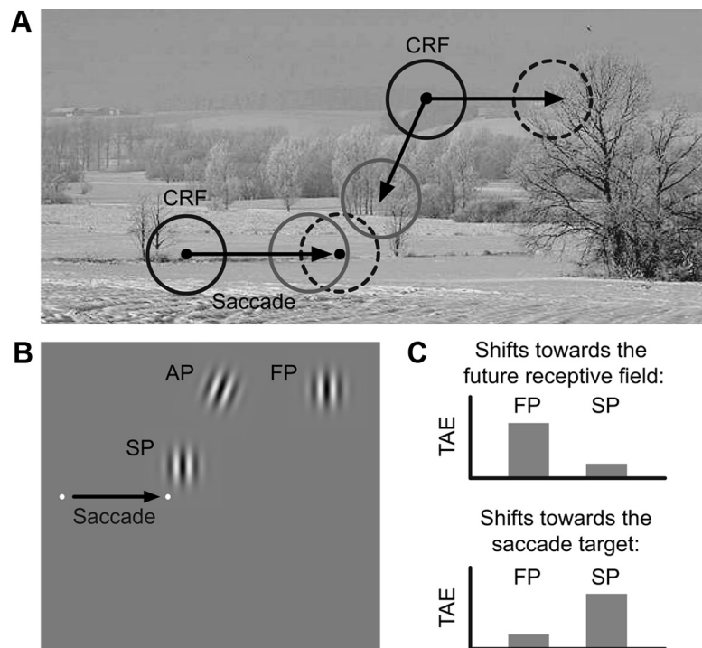
Figure 1. Hypothetical relationship between receptive field shifts and the tilt-aftereffect. A , Schematic illustration of two possible types of presaccadic receptive field dynamics. Two cells with their current receptive fields (CRF) are shown. For a current receptive field close to fixation, both types shift toward the future receptive field (black dashed circles), and shifts toward the saccade target (gray solid circles) are qualitatively similar and can hardly be distinguished since both change in the direction of the saccade. For a receptive field above the saccade target, both types can be dissociated since a presaccadic shift toward the future receptive field consists of a change in the direction of the saccade, whereas a shift toward the saccade target consists of a change orthogonal and against the saccade direction. Note the depicted receptive fields are intended to qualitatively illustrate the direction of the change in receptive field location and do not provide information about the absolute size. B , To the left, the spatial layout of stimuli used to measure the presaccadic tilt-aftereffect is shown. The position of the adaptor is abbreviated as AP, while FP and SP denote the future position and saccade target position, respectively. C , The two predictions for the tilt-aftereffect (TAE) made by shifts toward the future receptive field and shifts toward the saccade target. If a shift toward the future receptive field was true, the presaccadic tilt-aftereffect measured at the future position should be larger than the tilt-aftereffect at the saccade target position. In contrast, if a shift toward the saccade target was true, the tilt-aftereffect measured at the future position should be smaller than the tilt-aftereffect at the saccade target position.
