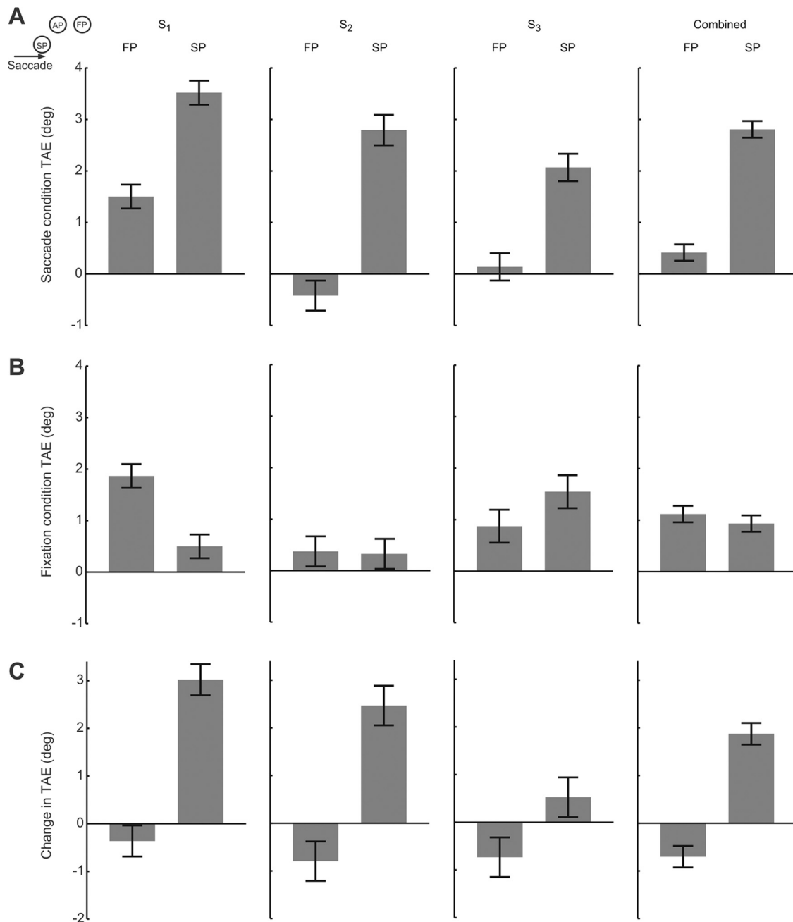
Figure 2. Results for the future position (FP) and the saccade target position (SP) for all single subjects ( S_1, S_2, S_3 ) and the combined data. A , Tilt-aftereffect (TAE) as measured immediately before a saccade. Error bars indicate SEs. The tilt-aftereffect is significantly stronger for all subjects and the combined data at the saccade target position. B , Tilt-aftereffect measured during continuous fixation serving as baseline. C , Difference of the tilt-aftereffect in the saccade and fixation condition. The tilt-aftereffect tends to increase at saccade target position and to decrease at the future position. This differential effect is significant for all subjects and the combined data.
