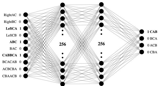
Figure 1: Neural network with the example task ABC/Left;C;A, encoded as a one-hot-encoded vector.
