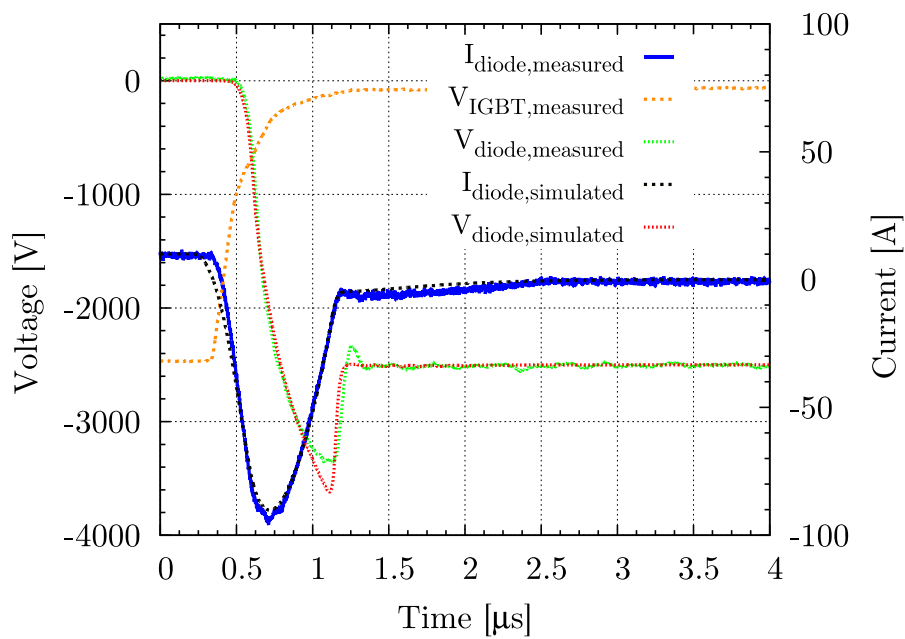
Measured and simulated turn-off behaviour of a 3.3kV CIBH diode
