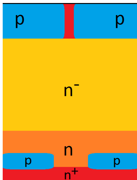
Simplified structure of an IDEE diode
