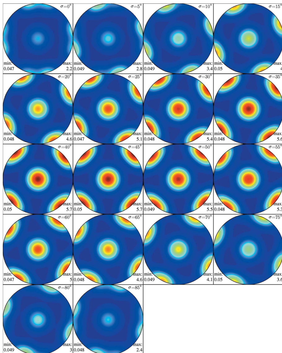
Figure 5 Estimated ODF after initial measurements.
