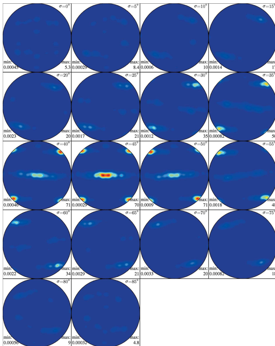
Figure 7 Estimated ODF after the second refinement.
