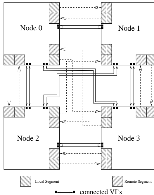
Figure 2: VIA/SCI device after initialization
