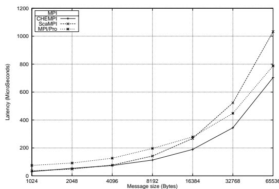
Figure 5: Ping-pong latency (half round-trip) between 2 MPI processes with message sizes 1KB .. 64KB
