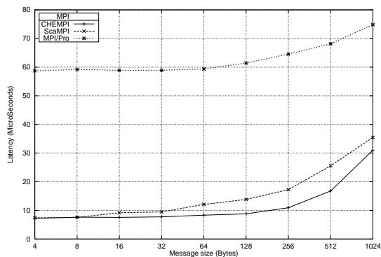
Figure 4: Ping-pong latency half round-trip between 2 MPI processes with message sizes 0Bytes .. 1024Bytes
