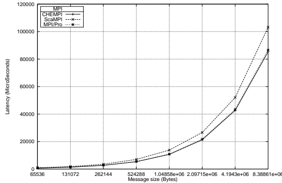
Figure 6: Ping-pong latency (half round-trip) between 2 MPI processes with message sizes 64KB .. 8MB
