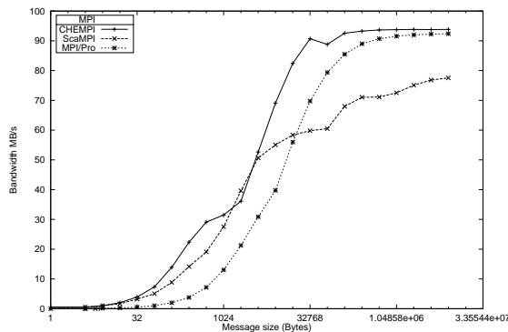
Figure 7: Ping-pong bandwidth (half round-trip) between 2 MPI processes
