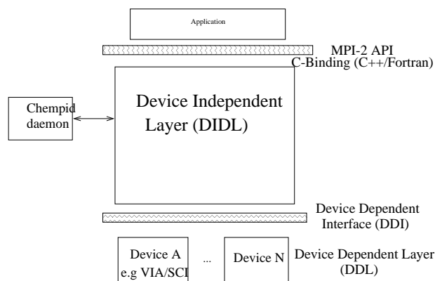
Figure 1: Raw structure of CHEMPI
