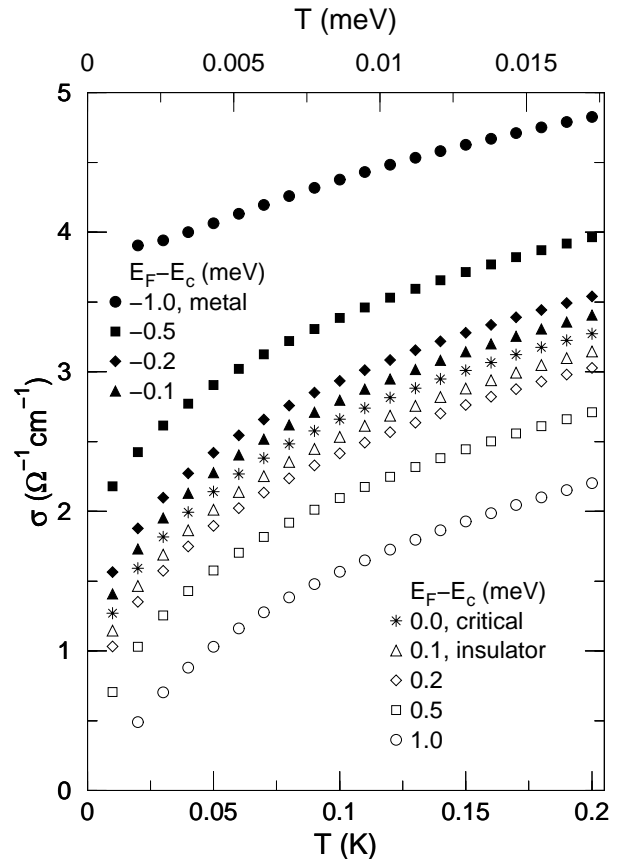
FIG. 1. Numerical calculations for the electrical conductivity, according to Eq. (5), as a function of temperature T . The filled symbols represent the metallic regime |E_F| < E_c , (*) denotes the critical regime E_F = E_c , and the open symbols represent the insulating regime |E_F| > E_c .
