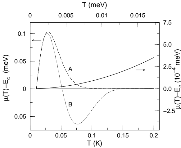
FIG. 5. Comparison between modified (dashed and dotted lines) and unmodified (solid lines) chemical potentials. The curves are shifted with respect to the mobility edge. The thick solid line is the unmodified \mu shown on a finer (right) scale.
