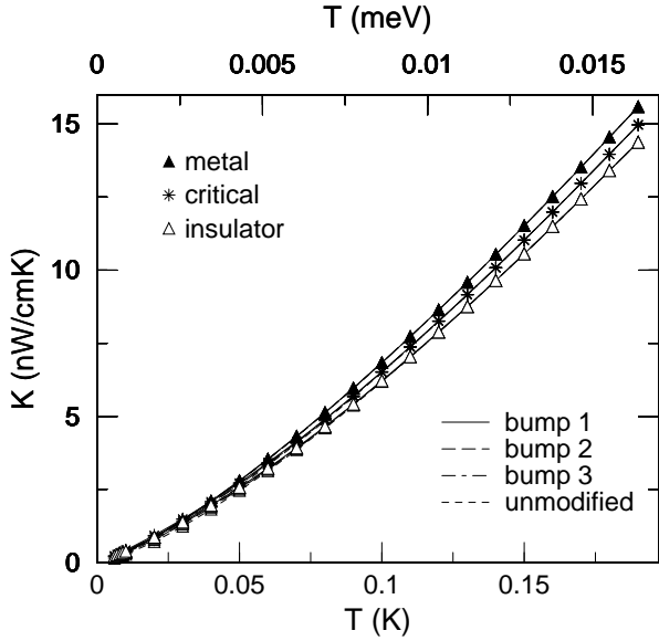
FIG. 9. The thermal conductivity remains largely unaffected by variations in \sigma_c(E, T) . The data for unmodified and modified \sigma_c(E, T) lie on top of each other. The lines are guides for the eye only.
