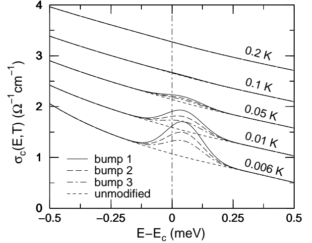
FIG. 6. The modified \sigma_c(E, T) as input having increasing bumps with decreasing T centered near at E - E_c = 0.05 meV. For clarity only selected isotherms are shown. The vertical line indicates the mobility edge.
