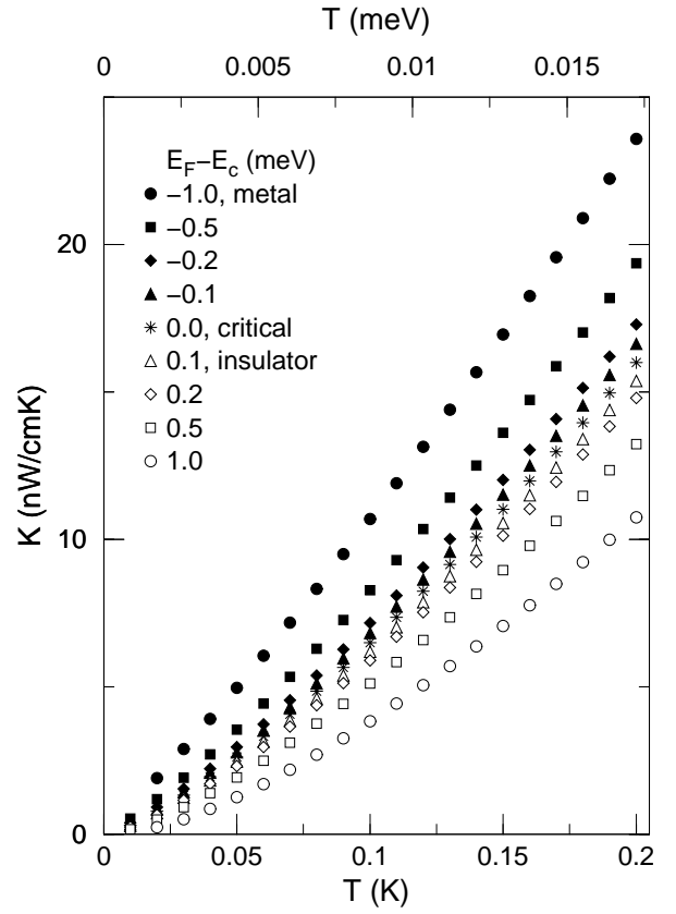
FIG. 3. The T dependence of the thermal conductivity computed with Eq. (8).
