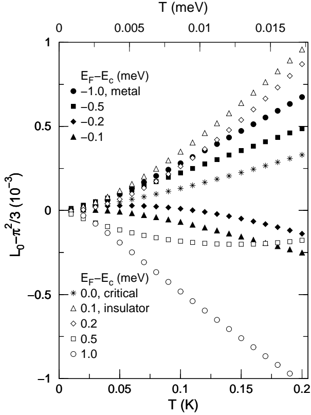
FIG. 4. The Lorenz number determined by Eq. (9). The results are shifted by \pi^2/3 , the universal value for metals. 31
