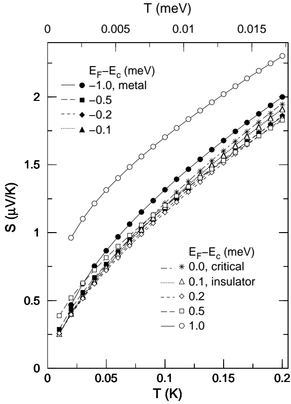
FIG. 2. The thermopower obtained from Eq. (6) as a function of T with the same symbols as in Fig. 1 distinguishing the metallic, critical and insulating regimes. The lines are obtained from Eq. (7).
