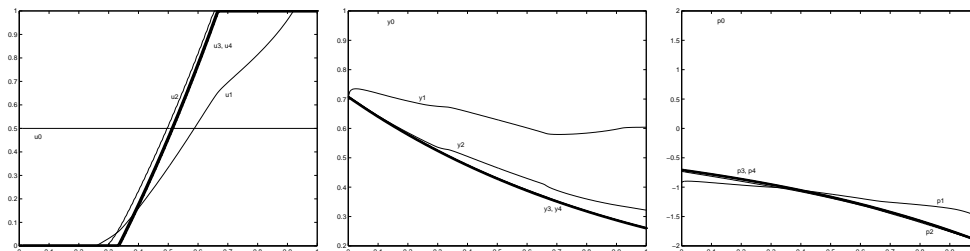
Figure 4: Controls, states, and adjoint states for Run 3
