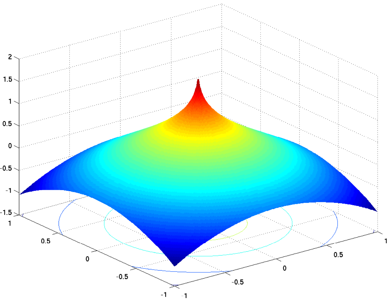
Plot of \log(|\log(r/2)|)
