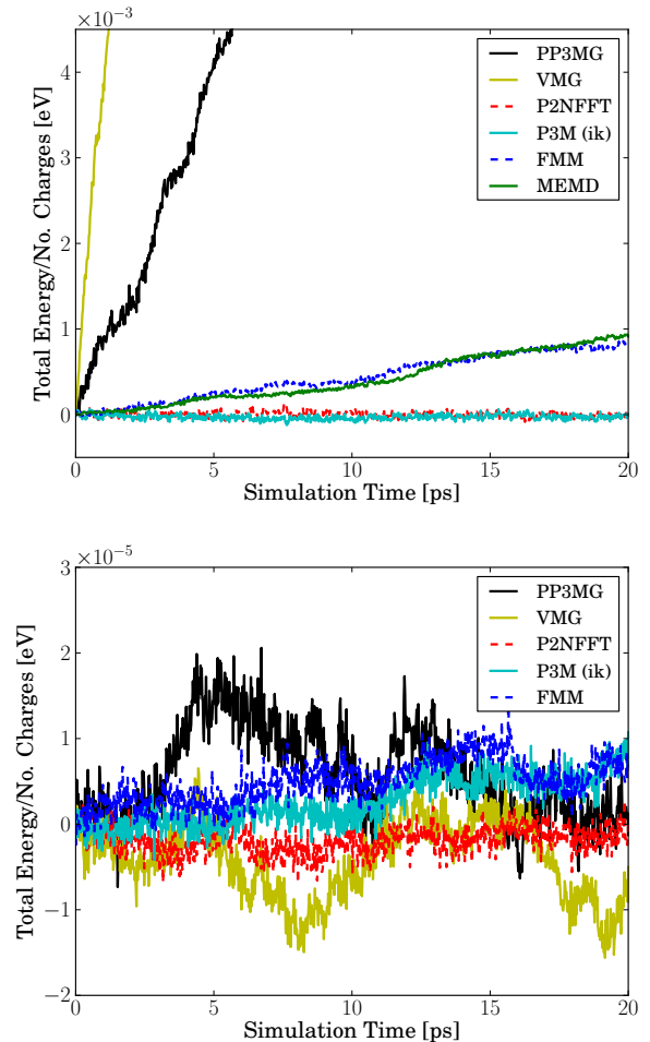
Figure 7. Total energy per particle according to different methods at accuracies \epsilon_{\text{pot}} = 10^{-3} (top) and \epsilon_{\text{pot}} = 10^{-5} (bottom). The initial energy has been subtracted in order to make the fluctuations and the drift better visible. Note the different scales of the two figures (units of 10^{-3} eV and 10^{-5} eV). Note that the P 3 M method used here uses an ik -differentiation for the forces instead of analytical differentiation and does not apply interlacing. With MEMD, only an accuracy of \epsilon_{\text{pot}} = 10^{-3} could be reached.
