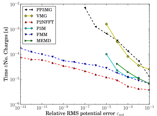
Figure 8. Required wall clock time per particle for 102 900 charges versus the relative rms potential error \varepsilon_{\text{pot}} on one core of JUROPA.
