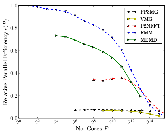
(b) Cloud-wall test case with 9830400 charges. t_{\text{best}} = 454.8\text{s} ; P_{\text{min}} = 2 .
