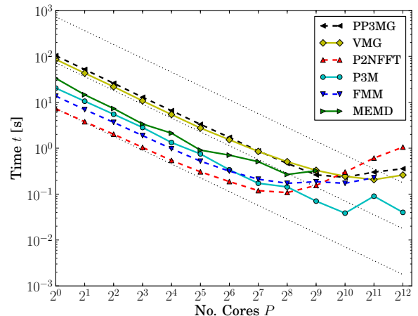
Figure 10. Required wall clock time of the cloud-wall test case with 1 012 500 charges versus the number of cores on JUROPA at relative rms potential error \varepsilon_{\text{pot}} < 10^{-3} .
