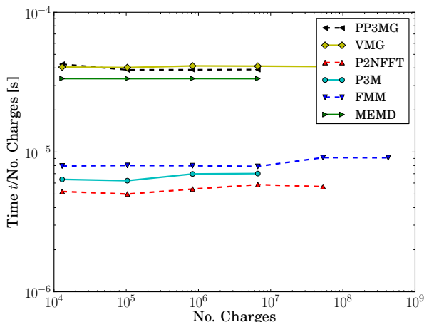
Figure 9. Required wall clock time per particle at relative rms potential error \varepsilon_{\text{pot}} < 10^{-3} on one core of JUROPA.
