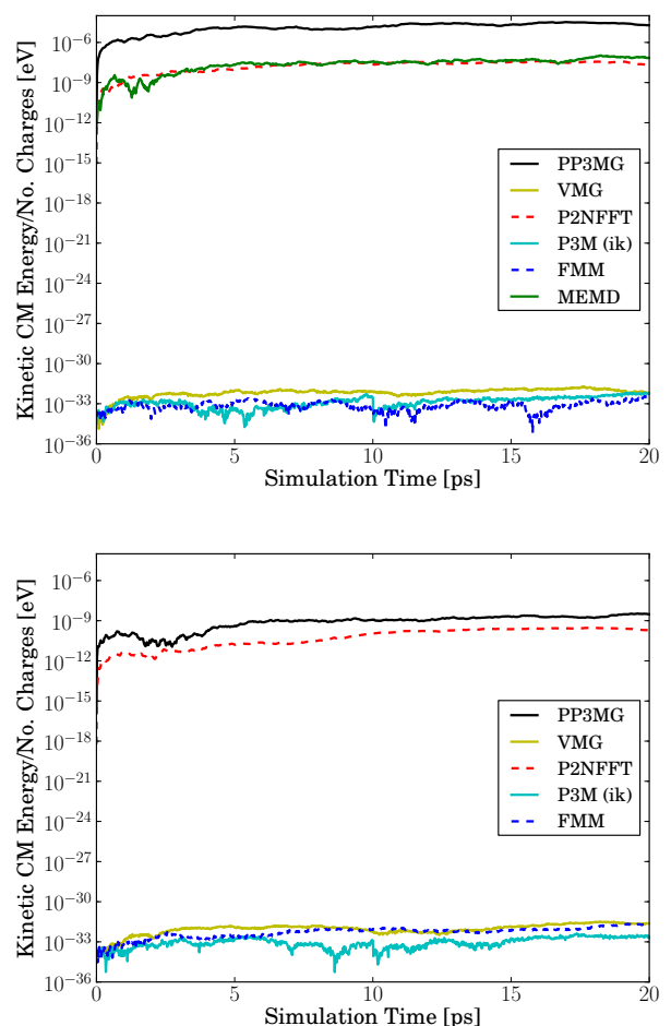
Figure 6. Kinetic energy per particle of the center-of-mass motion of the system according to different methods and accuracies: \varepsilon_{\text{pot}} = 10^{-3} (top); \varepsilon_{\text{pot}} = 10^{-5} (bottom). Note that the P 3 M method used here uses an ik -differentiation for the forces instead of analytical differentiation and does not apply interlacing. With MEMD, only an accuracy of \varepsilon_{\text{pot}} = 10^{-3} could be reached.
