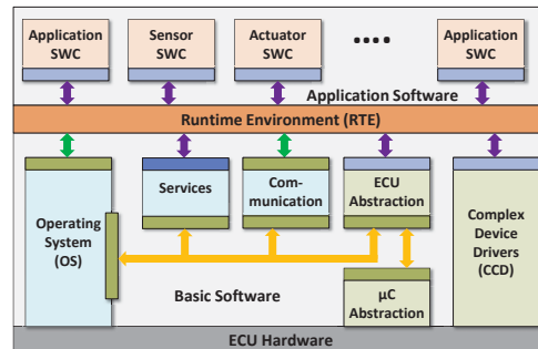
Figure 1: AUTOSAR software layers
